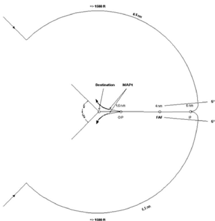
Figure 2 of GM OPS.CAT.150.H Base Turn Procedure – Direct Approach
