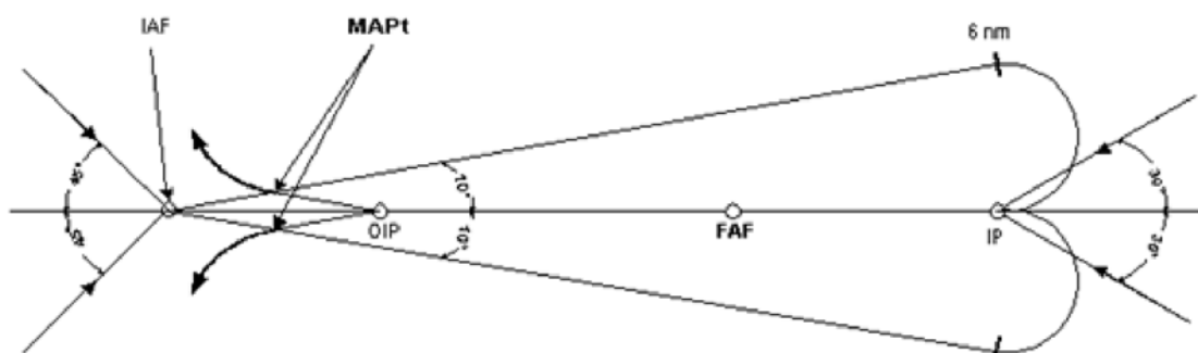
Figure 3 of GM OPS.CAT.150.H Holding Pattern & Race Track Procedure
