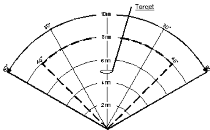
Figure 5 of GM OPS.CAT.150.H Missed Approach Area Left &amp; Right
