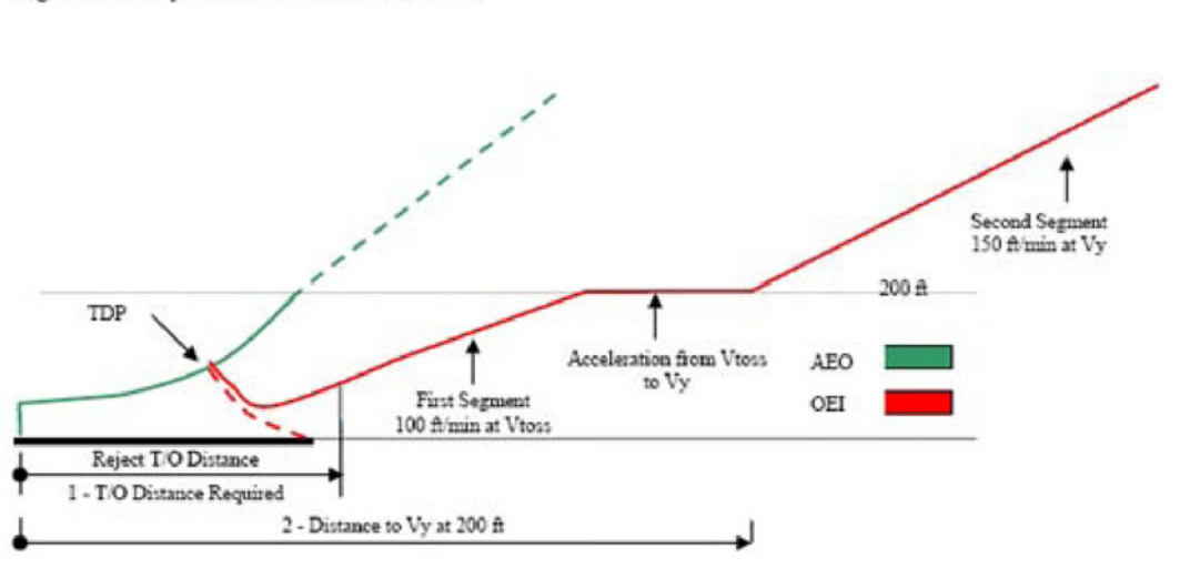
Figure 2 - Performance Class 1 distances
